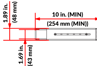
SIDE VIEW (MIN)
