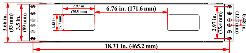
FRONT VIEW
