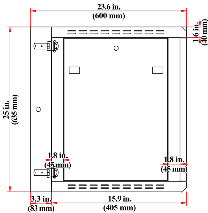
SIDE VIEW
