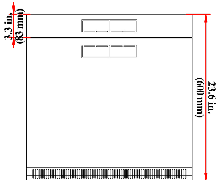
BOTTOM VIEW
