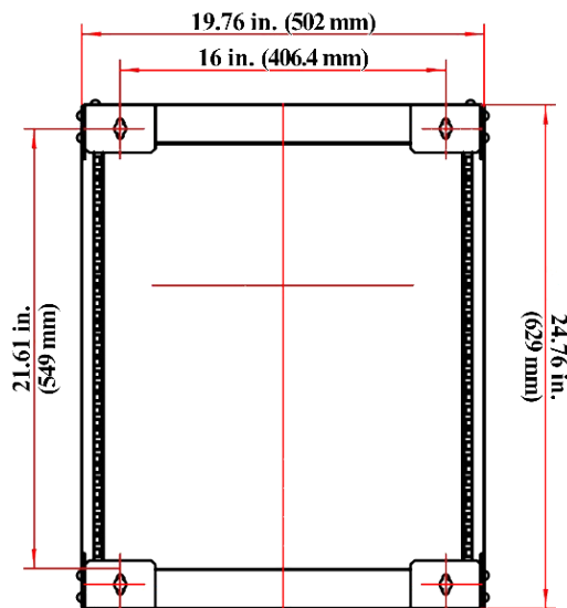
REAR VIEW
