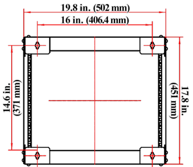
REAR VIEW
