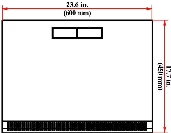
BOTTOM VIEW
