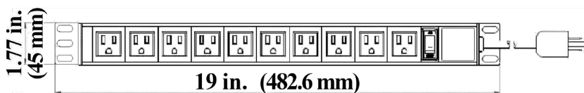
TOP VIEW
