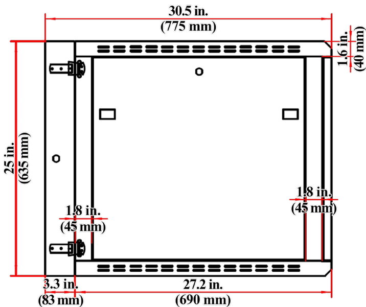
SIDE VIEW
