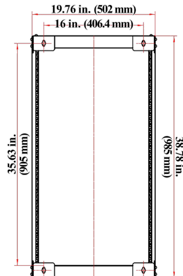
REAR VIEW
