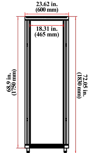
INSIDE VIEW
