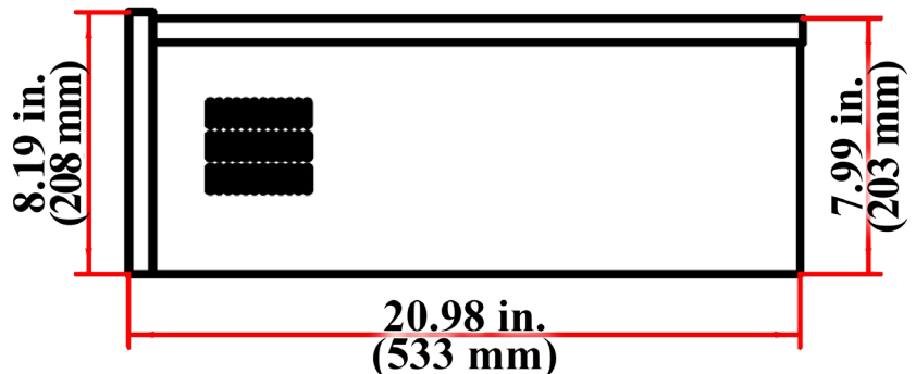
SIDE
