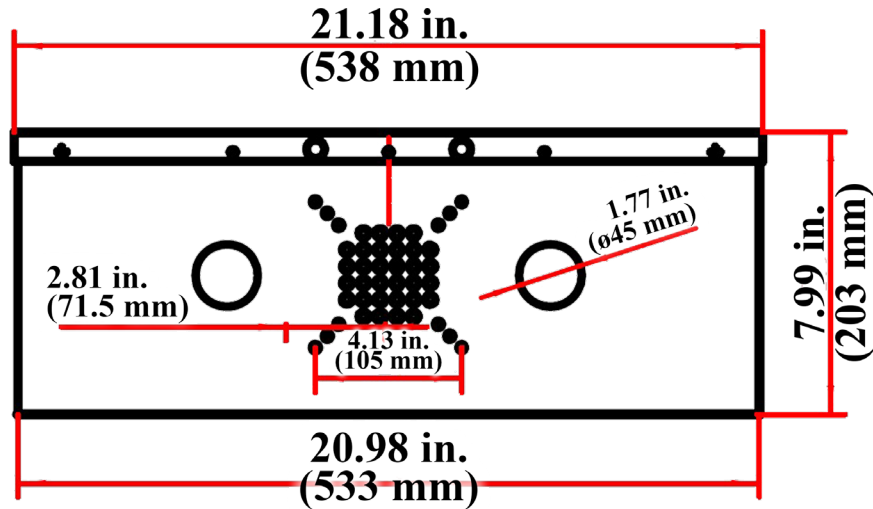
REAR SIDE
