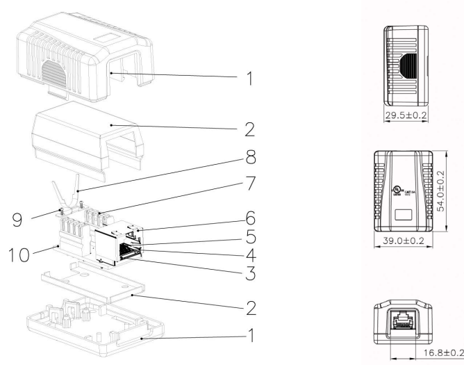
CAT6A Surface Mount Box Diagrams
