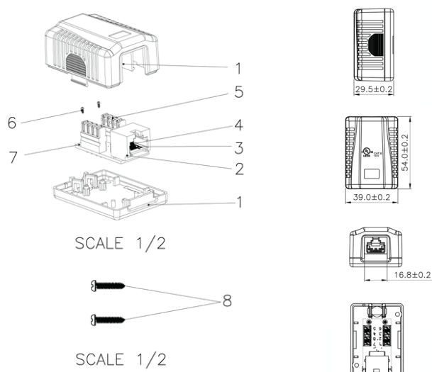
CAT5E & CAT6 Surface Mount Box Diagrams
