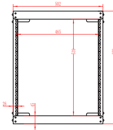
FROM FRONT
