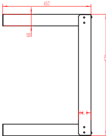
FROM SIDE
