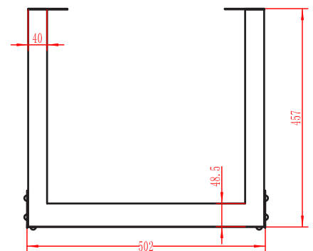
FROM TOP
