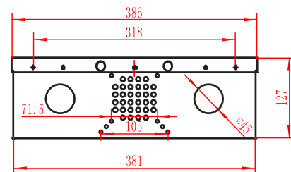
REAR SIDE
