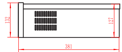
SIDE
