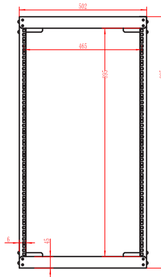
FROM FRONT
