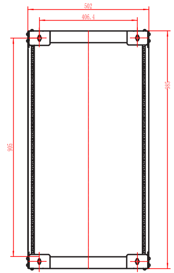
FROM REAR
