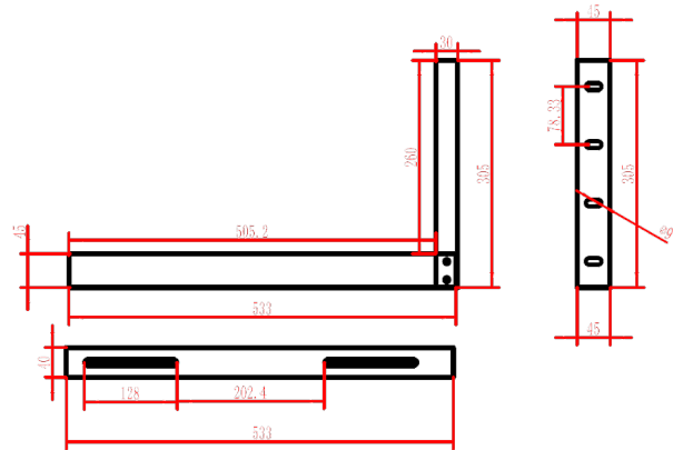
DVR HORIZONTAL WALLMOUNT BRACKET
